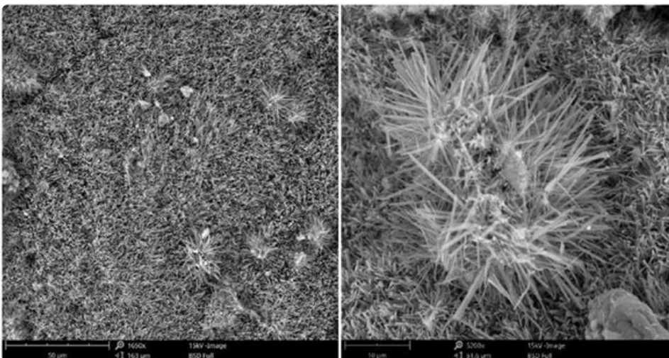
Scanning electron microscope images of MOC showing the needle-like phases of the binding mechanism. Author provided
